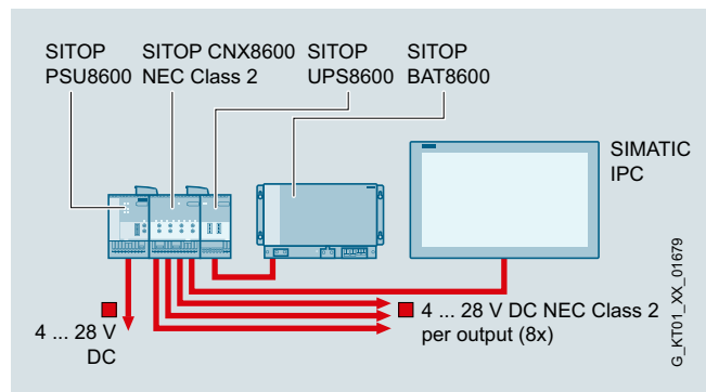
SIMATIC IPC power supply via SITOP PSU8600 power supply system with expansion module CNX8600 with NEC Class 2 and buffering of outputs by UPS8600 DC UPS with BAT8600 battery module
